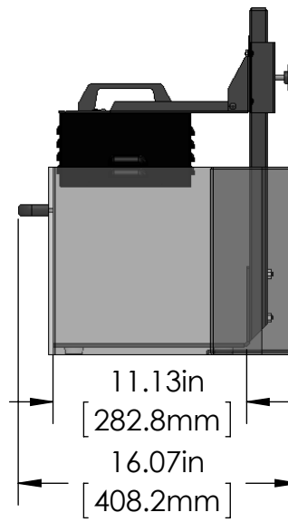
SIDE VIEW WITH REAR SHIELD
