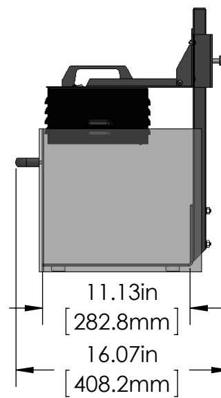
SIDE VIEW WITHOUT REAR SHIELD
